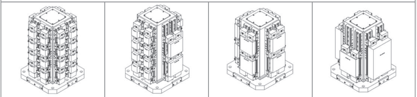
Illustrations show the various arrangements of workpieces possible with the custom Triag tombstone-type workholding devices provided by AME to TRD Mfg. for the production of cylinder heads and caps.
