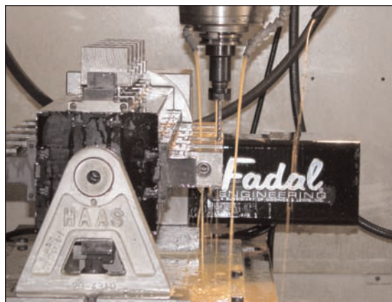
Triag compact clamping system with integral trunnion from Advanced Machine & Engineering, for use with any rotary indexer; allows continuous three-sided machining and thereby reduces handling and cycle times
