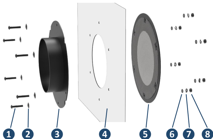
Fig. 1: Installing the hose flange on the machine tool
