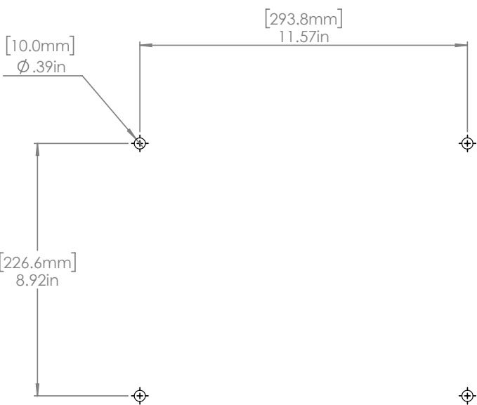
Fig 23: Floor mount bolt pattern
