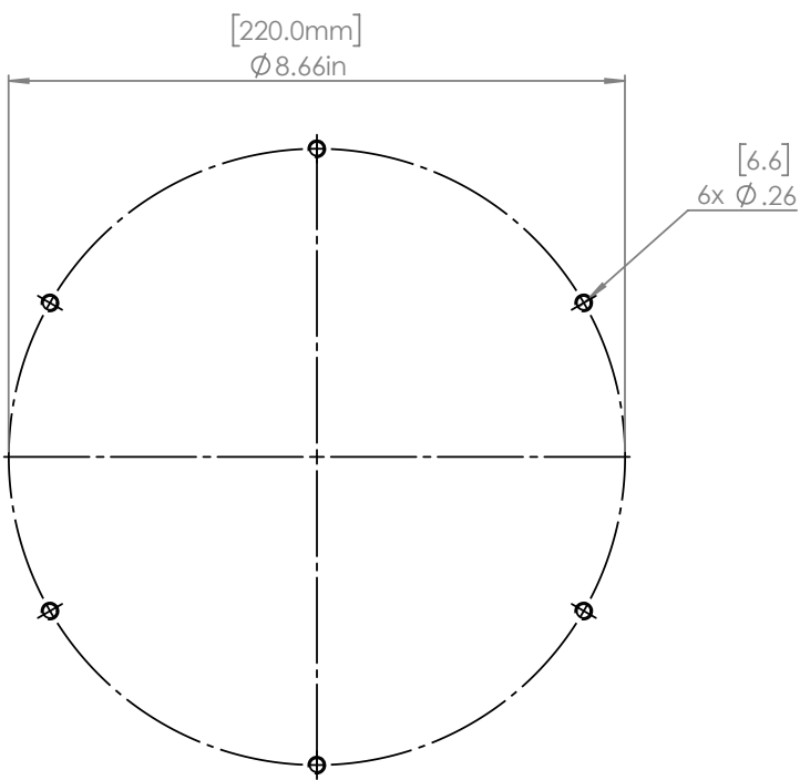
Fig 21: Hose flange bolt pattern
