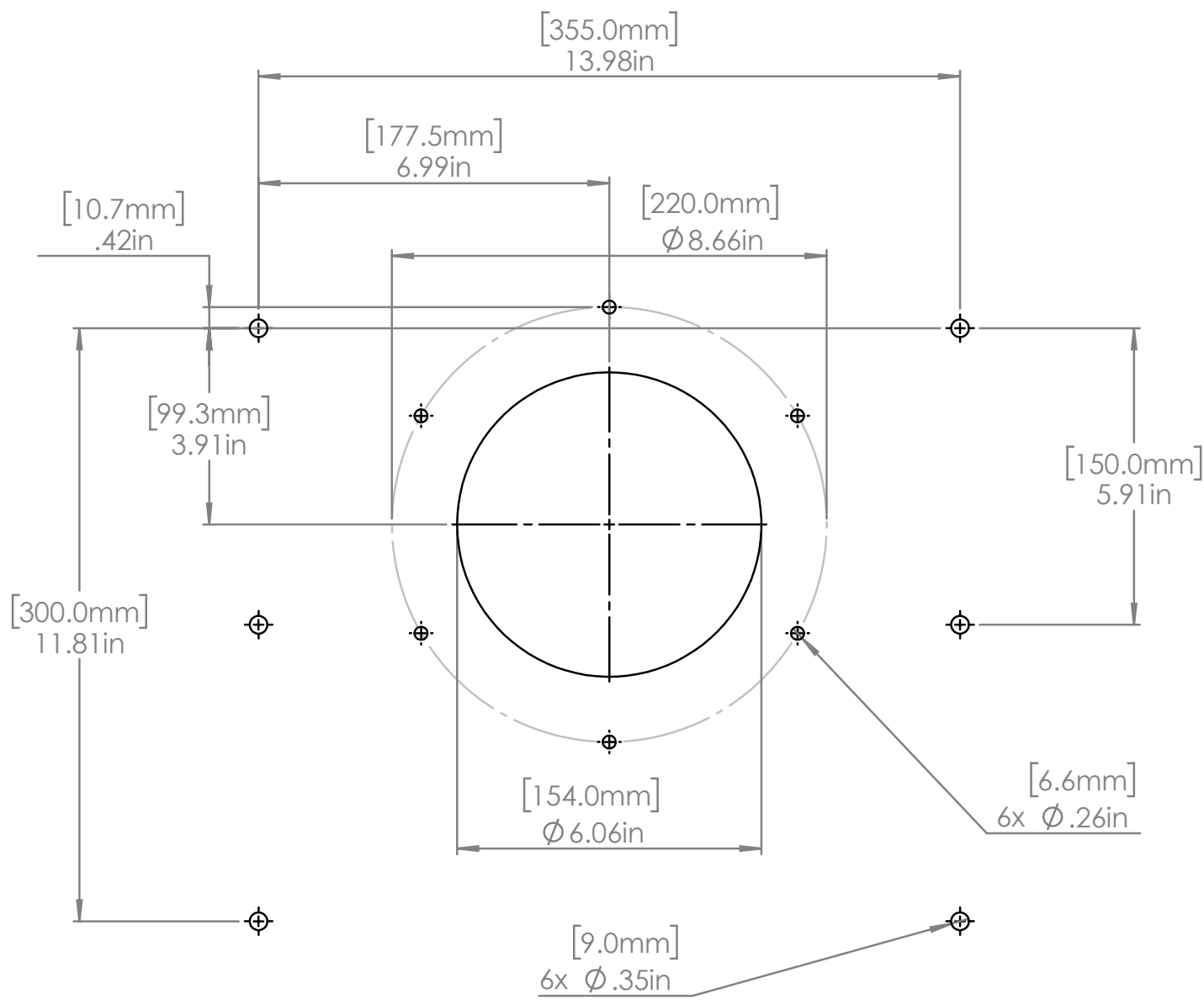
Fig 24: Side mount and hose flange bolt pattern
