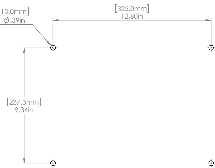
Fig 22: Universal mount bolt pattern
